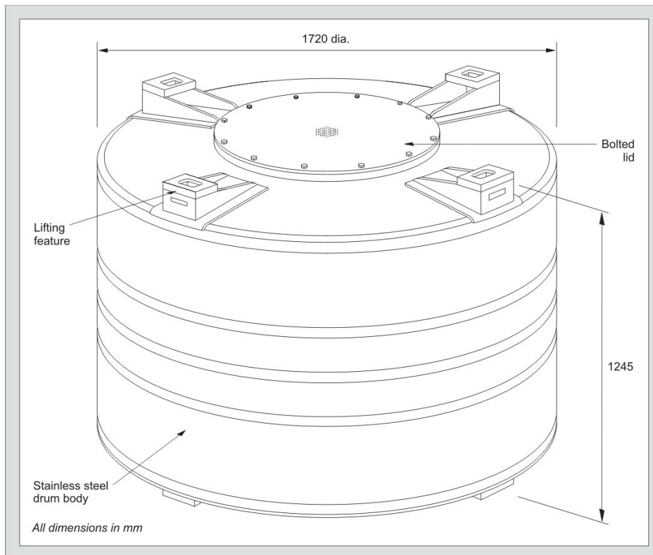
Figure 3 3 cubic metre Drum Waste Package
