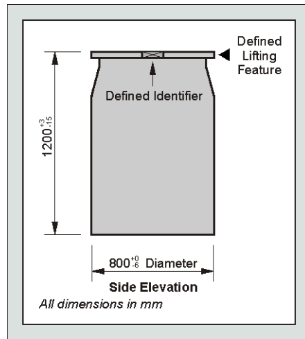
Figure 3 Standard Lifting Feature for 500 litre Drum Waste Package
