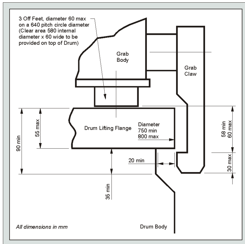
Figure 3 Standard Lifting Feature for 500 litre Drum Waste Package
